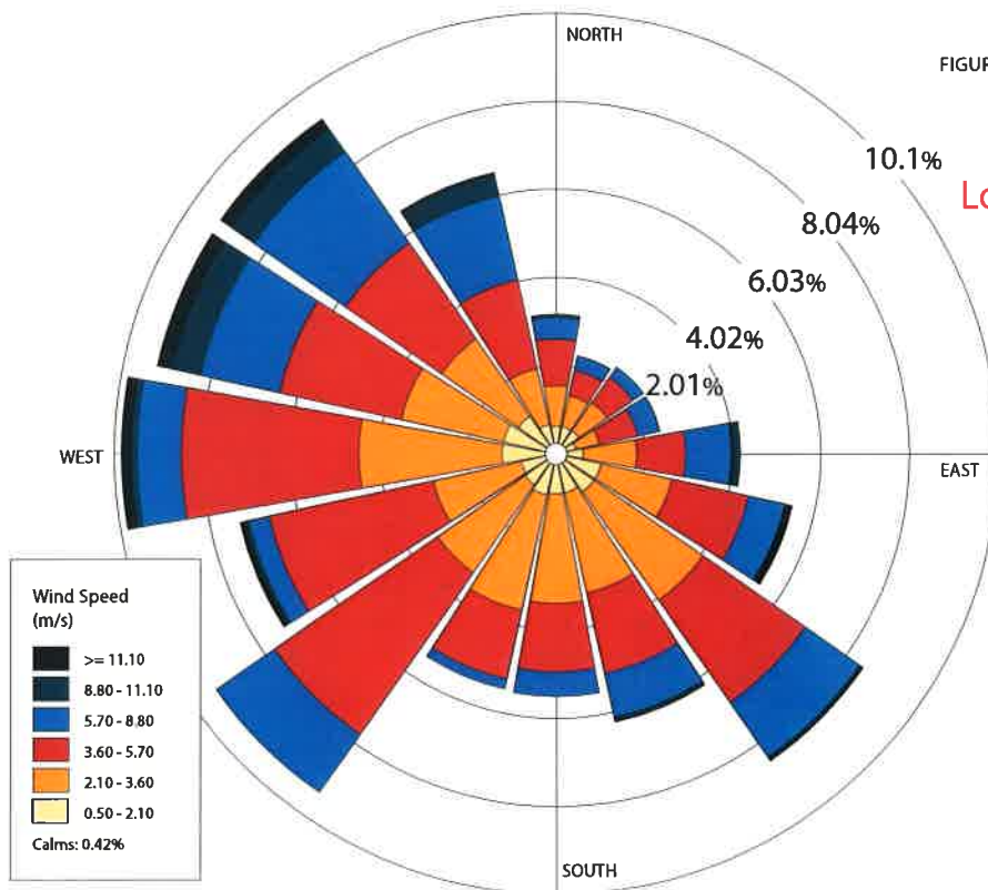
FIGURE 5. Wind Rose for 2018 Calendar Year
