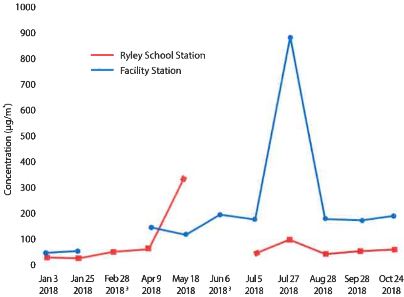
FIGURE 3. 2018 Particulate Concentrations
